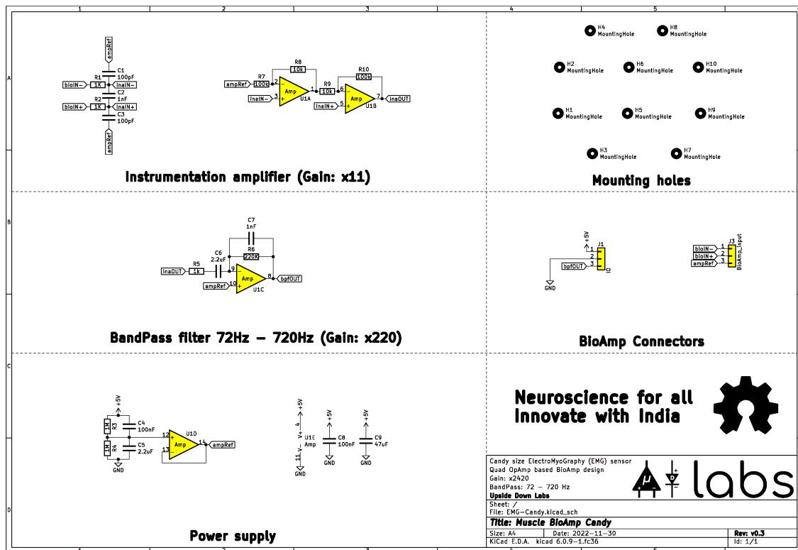
Fig. 6: Schematic Diagram
