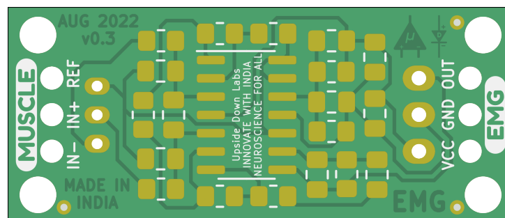
Fig. 1: PCB Front
